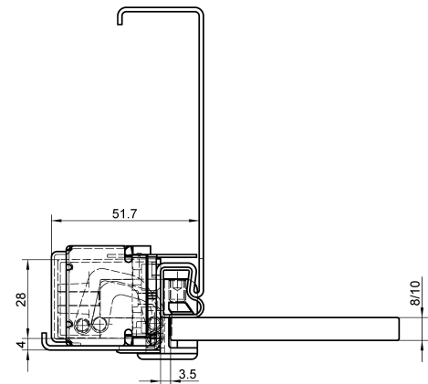
steel frame
