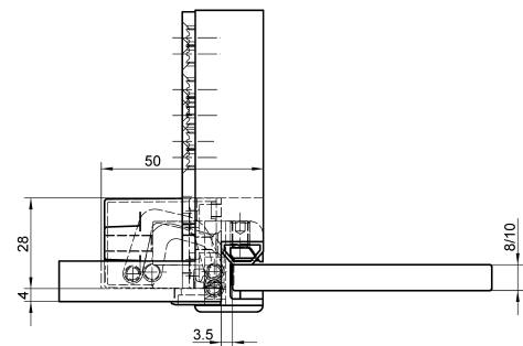
casing frame
